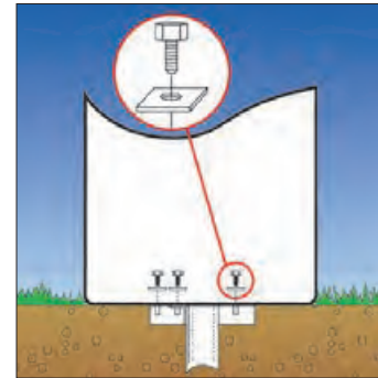
Internal view of litter bin showing bolt fixing to Ground-Lock system.
